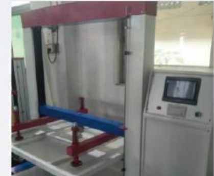
Compression Tester
