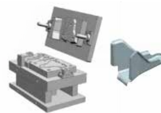
Exhaust system component stamping die
