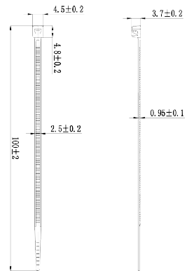
Cable Tie 2.5* 100mm Color: Custom
