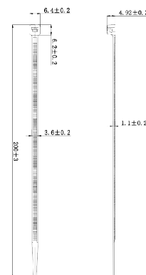
Cable Tie 3.6*200mm Color: Custom
