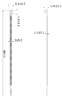
CableTie3.0*200mm Color: Custom
