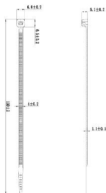
Cable Tie 4.0*150mm Color: Custom
