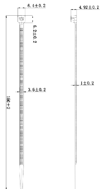
Cable Tie 3.6*150mm Color: Custom
