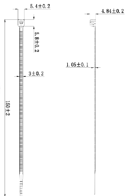
Cable Tie 3.0 150mm Color: Custom
