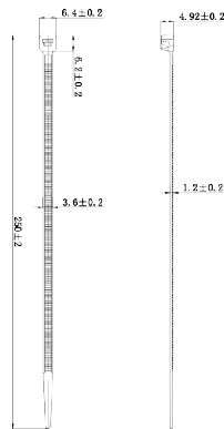
Cable Tie 3.6*250mm Color: Custom
