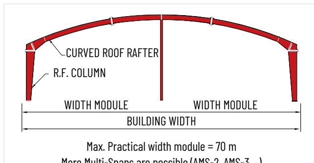
Arched Multi-Span (AMS-1)
