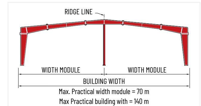
Multi-span "1" (MS-1)
