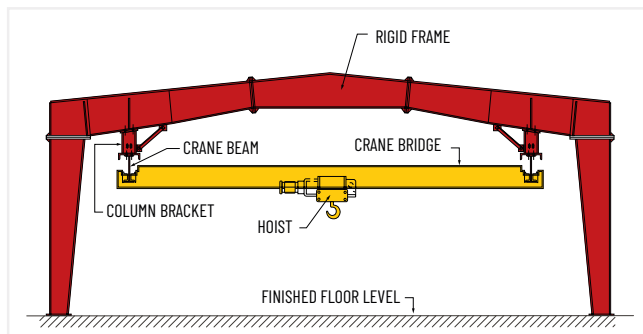
Underhung Crane
