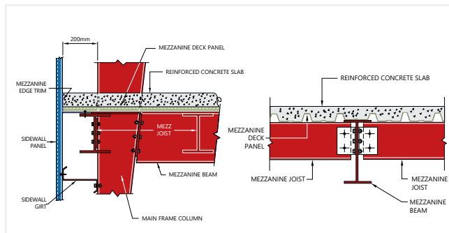
Mezzanine detail
