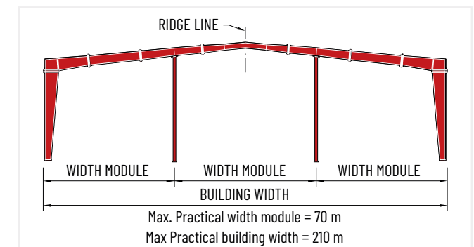
Multi-Span"2" (MS-2)
