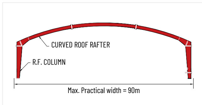
Arched Clear-Span (AS)
