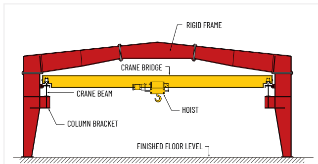
Top Running Crane
