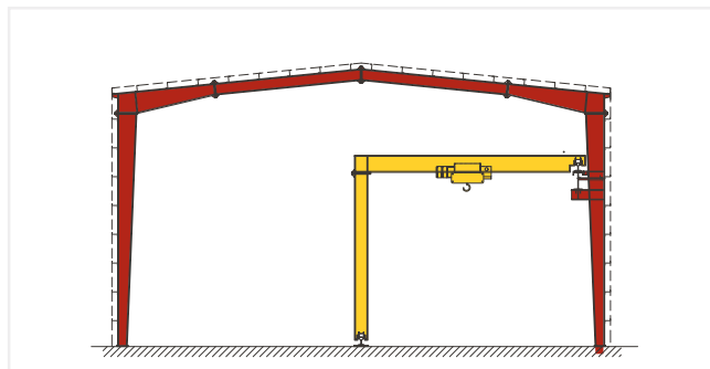
Semi Portal Crane
