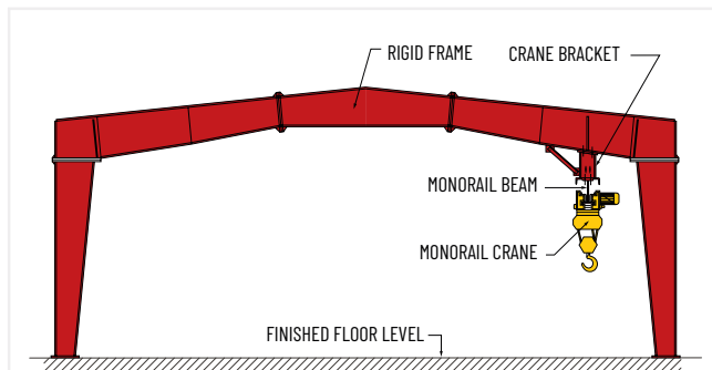
Monorail Crane
