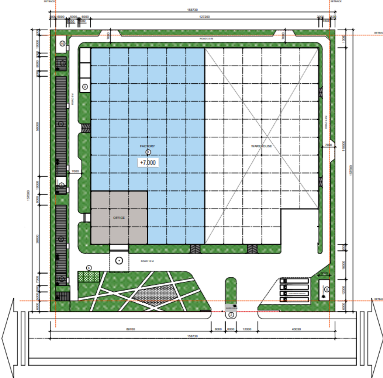
MEZZANINE MASTER PLAN SCALE: 1/500
