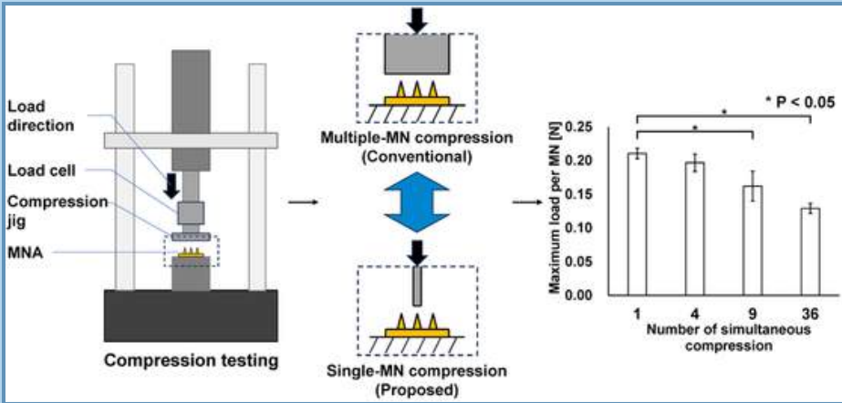
Compression Test
